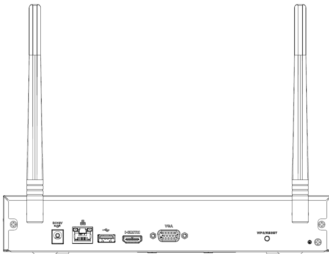
Figura 2-56 Panel trasero
