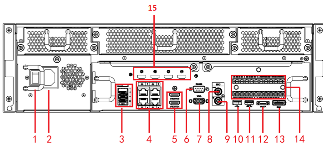
Figura 2-78 Panel trasero
