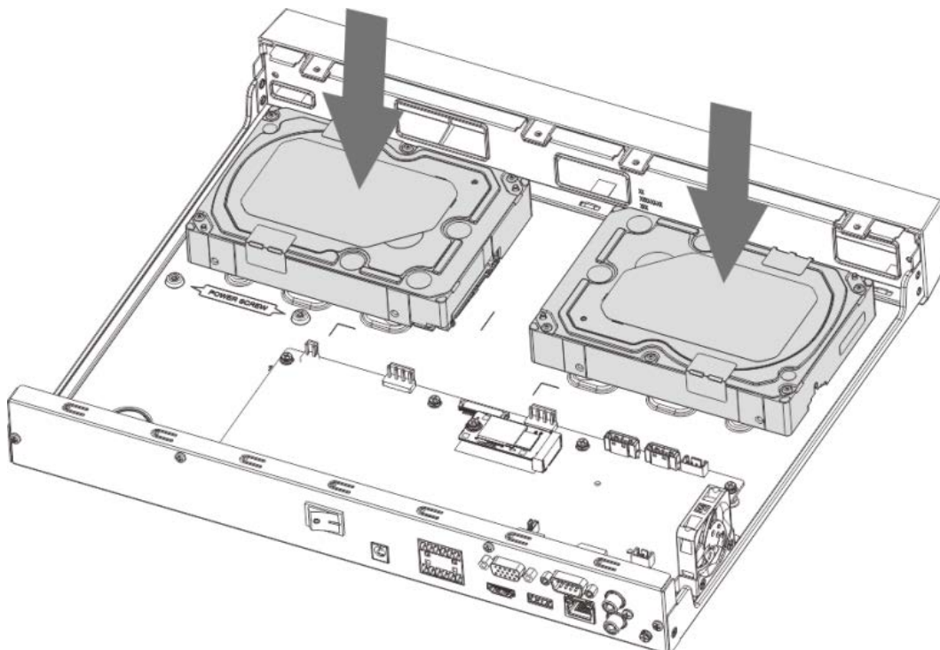
Figura 3-14 Alinear HDD
