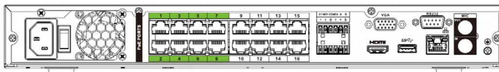
Figura 2-38 Panel trasero
