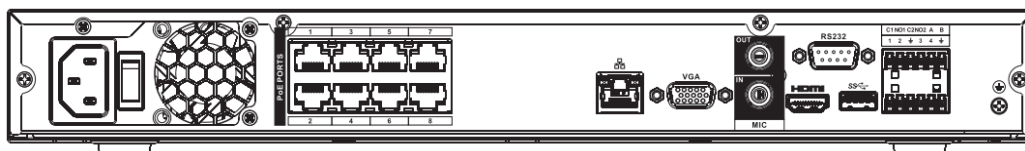
Figura 2-35 Panel trasero
