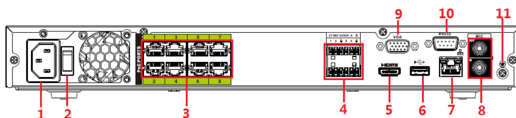
Figura 2-72 Panel trasero
