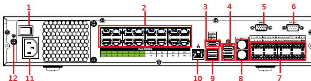
Figura 2-70 Panel trasero
