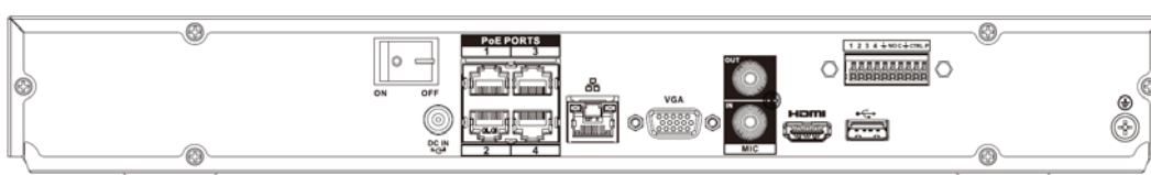
Figura 2-48 Panel trasero
