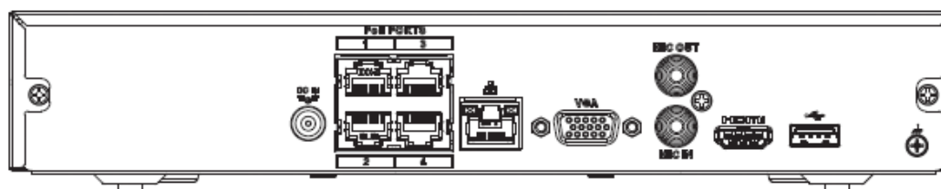
Figura 2-29 Panel trasero
