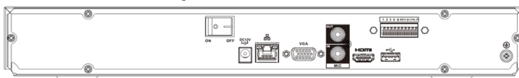
Figura 2-47 Panel trasero
